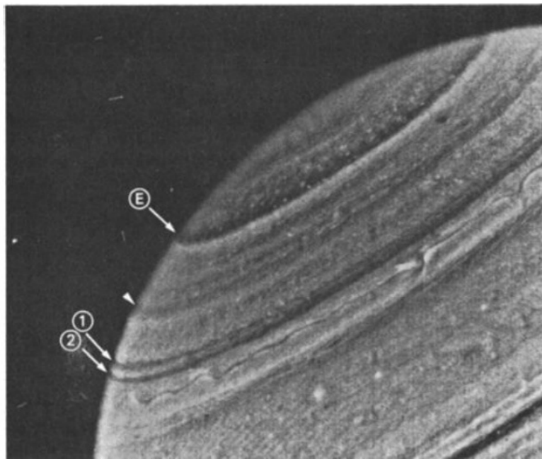
Fig. 2. Voyager 2 high contrast (green) image of Saturn's northern hemisphere.
